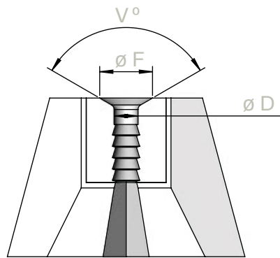
Countersunk
